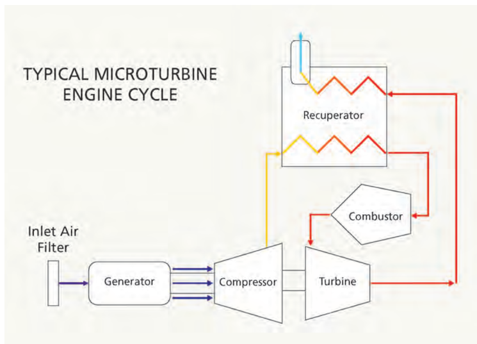
FIGURE 7: Microturbine Schematic
