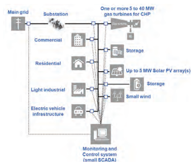
FIGURE 3: Microgrid Concept
